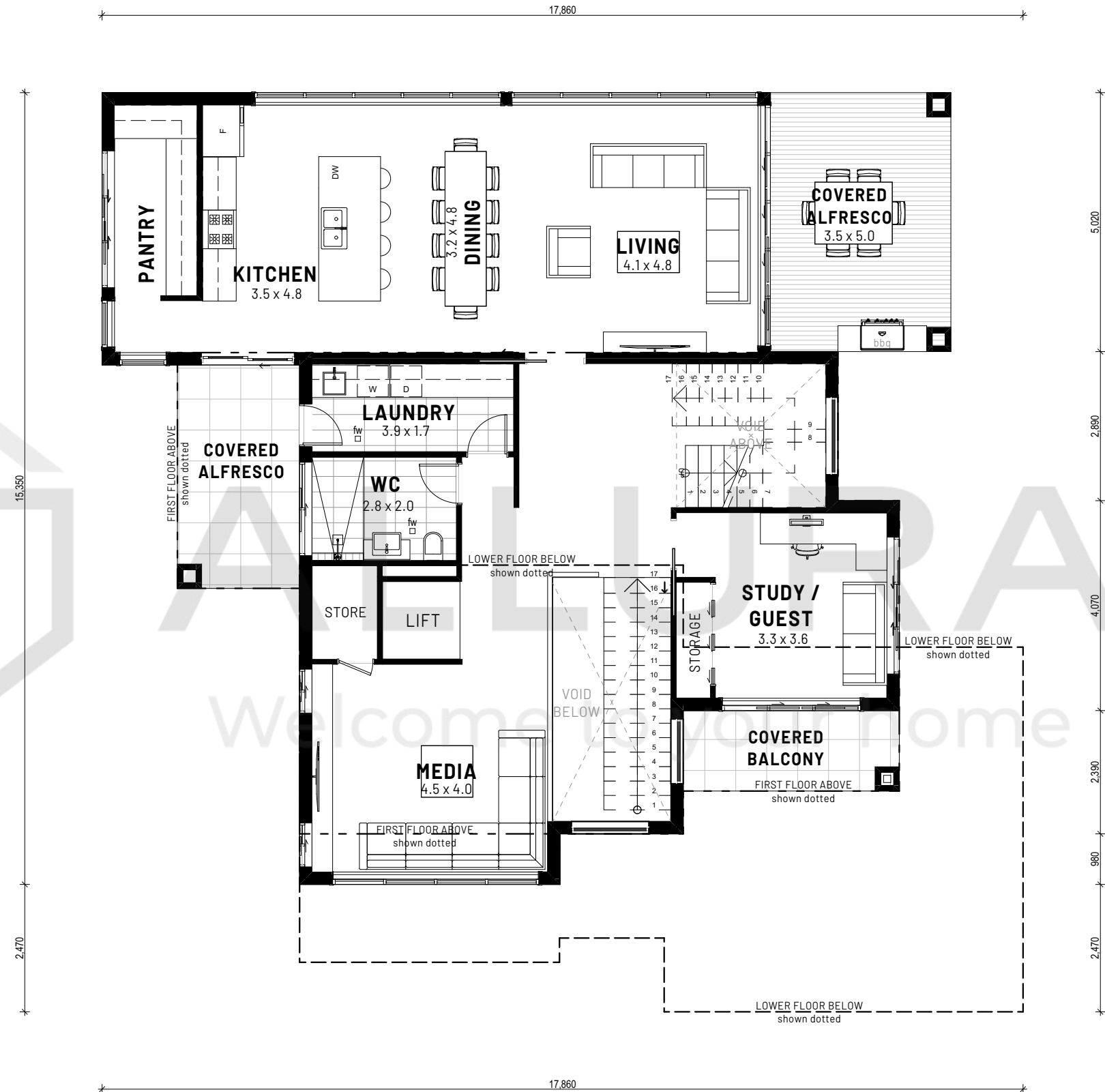
1 FIRST FLOOR PLAN 1:100
