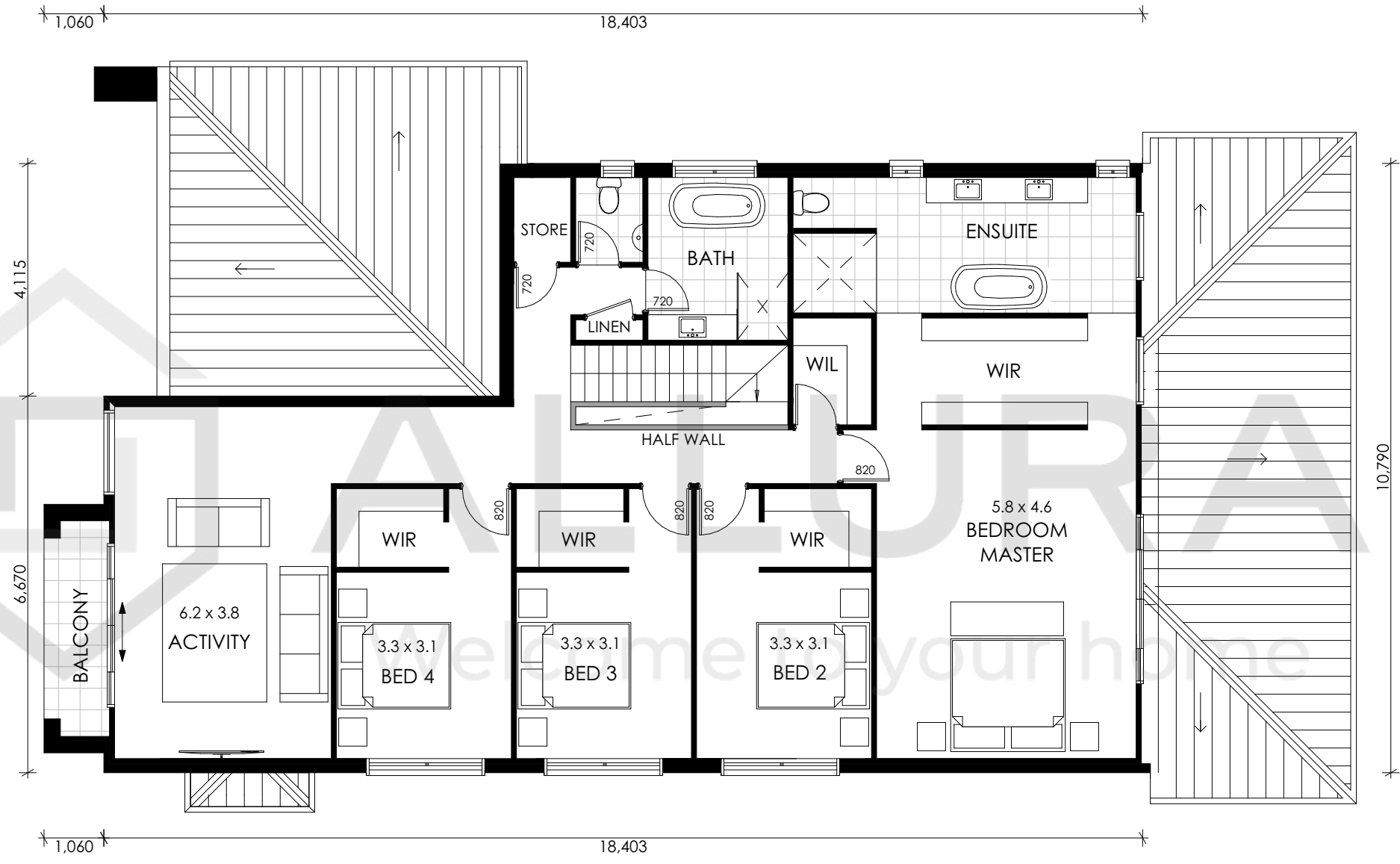
1 FIRST FLOOR PLAN 1:100
