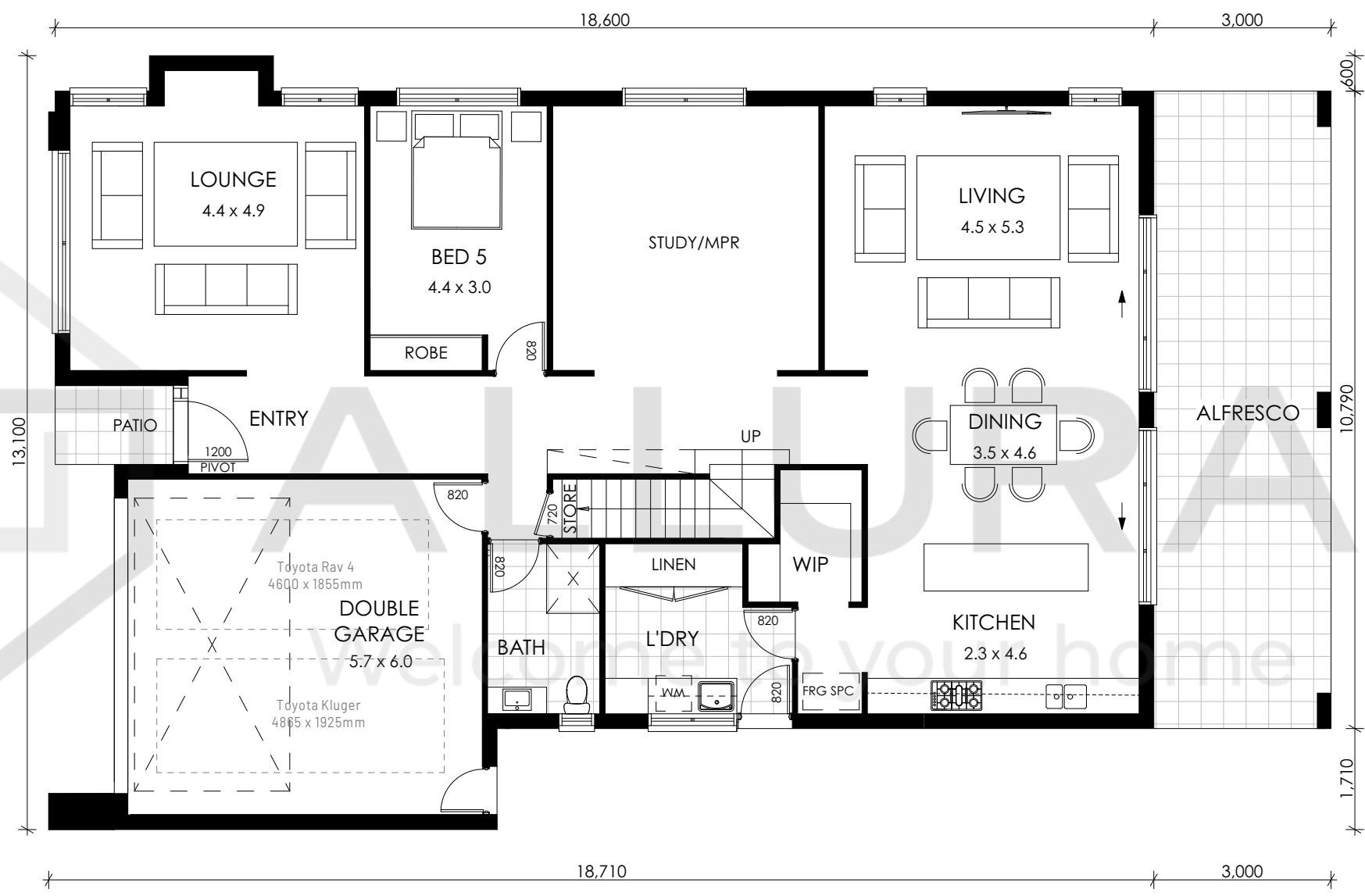
1 GROUND FLOOR PLAN 1:100
