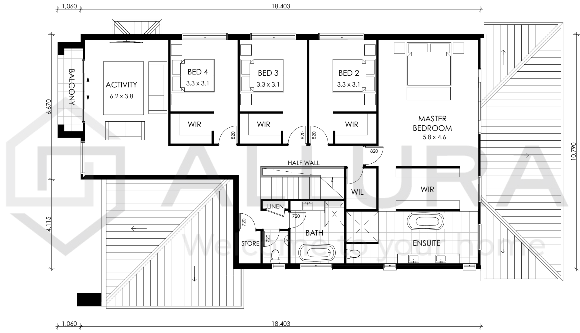
1 FIRST FLOOR PLAN 1:100
