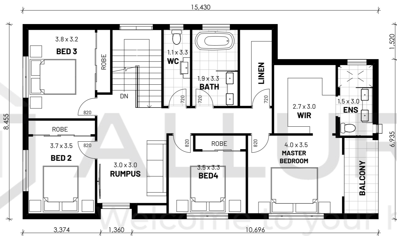
1 FIRST FLOOR PLAN 1:100
