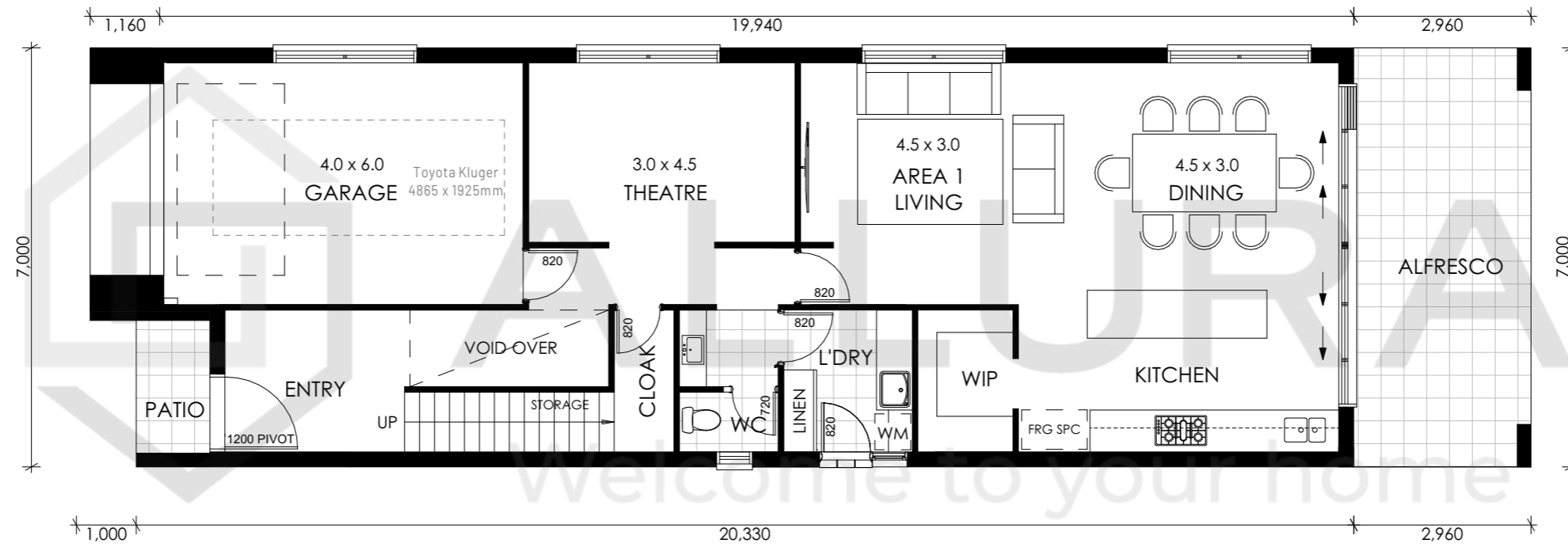
A3 GROUND FLOOR PLAN 1:100
