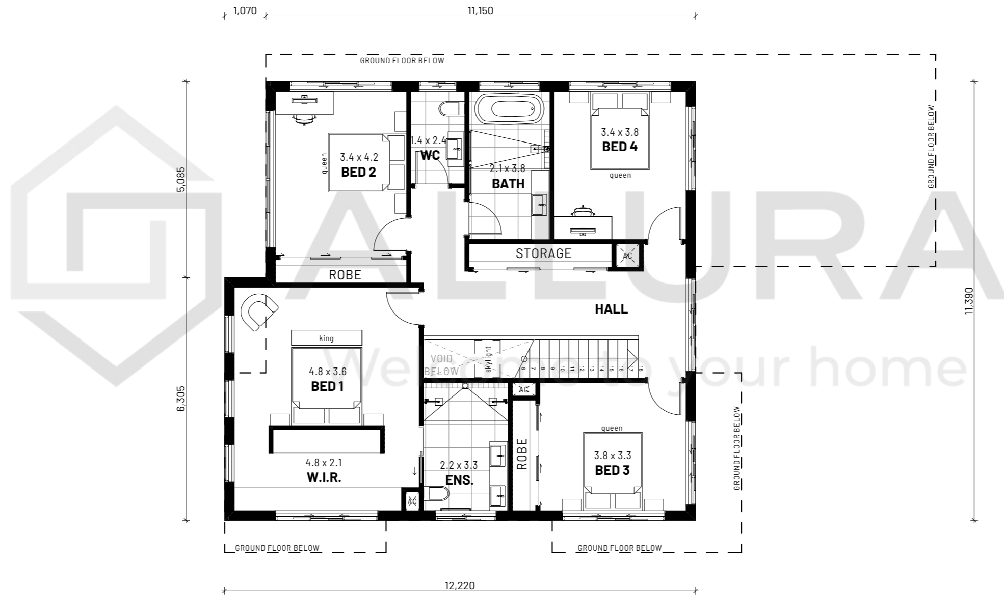
1 FIRST FLOOR PLAN - 1:100
