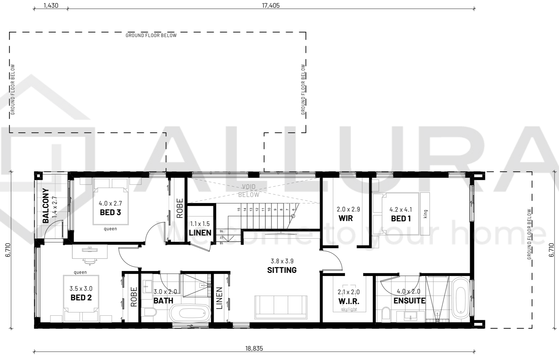
1 FIRST FLOOR PLAN - 1:100
